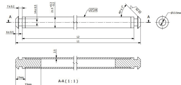
Full Hollow Axles with Close Ends
